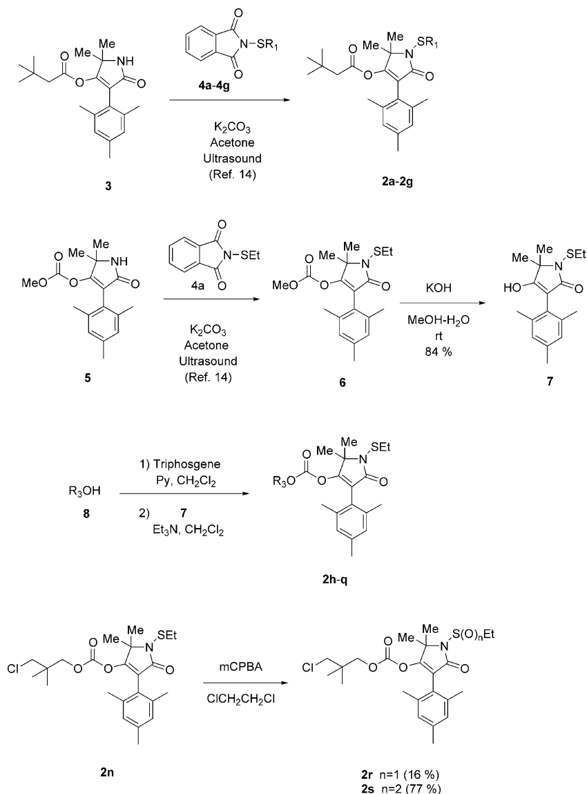
Scheme 1. Synthetic routes to novel dihydropyrrole derivatives with N -sulfanyl, sulfinyl, and sulfonyl moieties.
